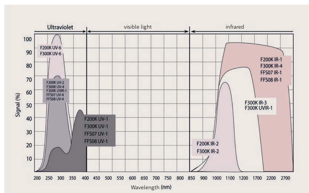
Fig. Sensor signal as a dependence on wavelength
