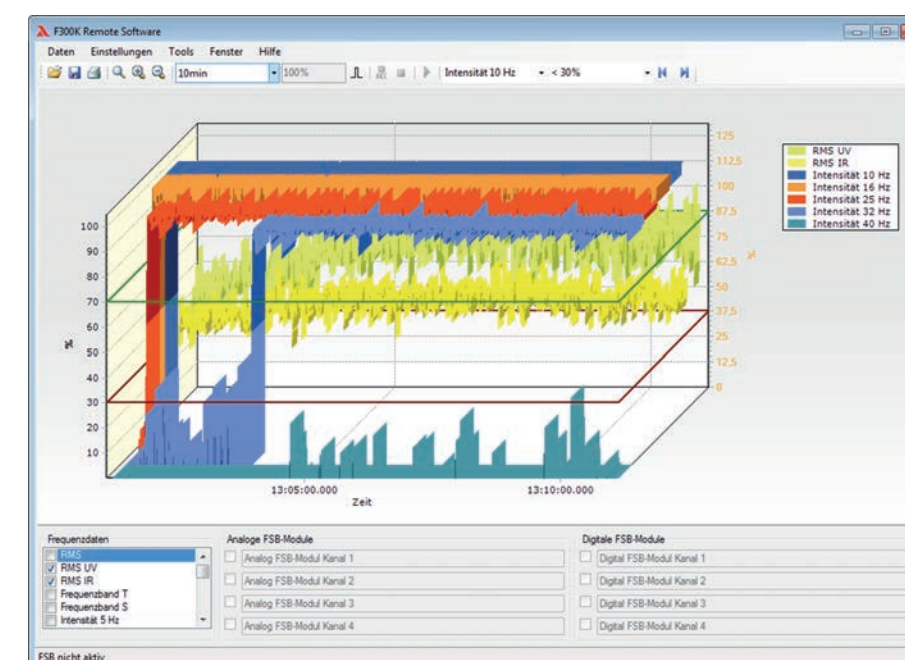
Fig. Flame analysis F300K
