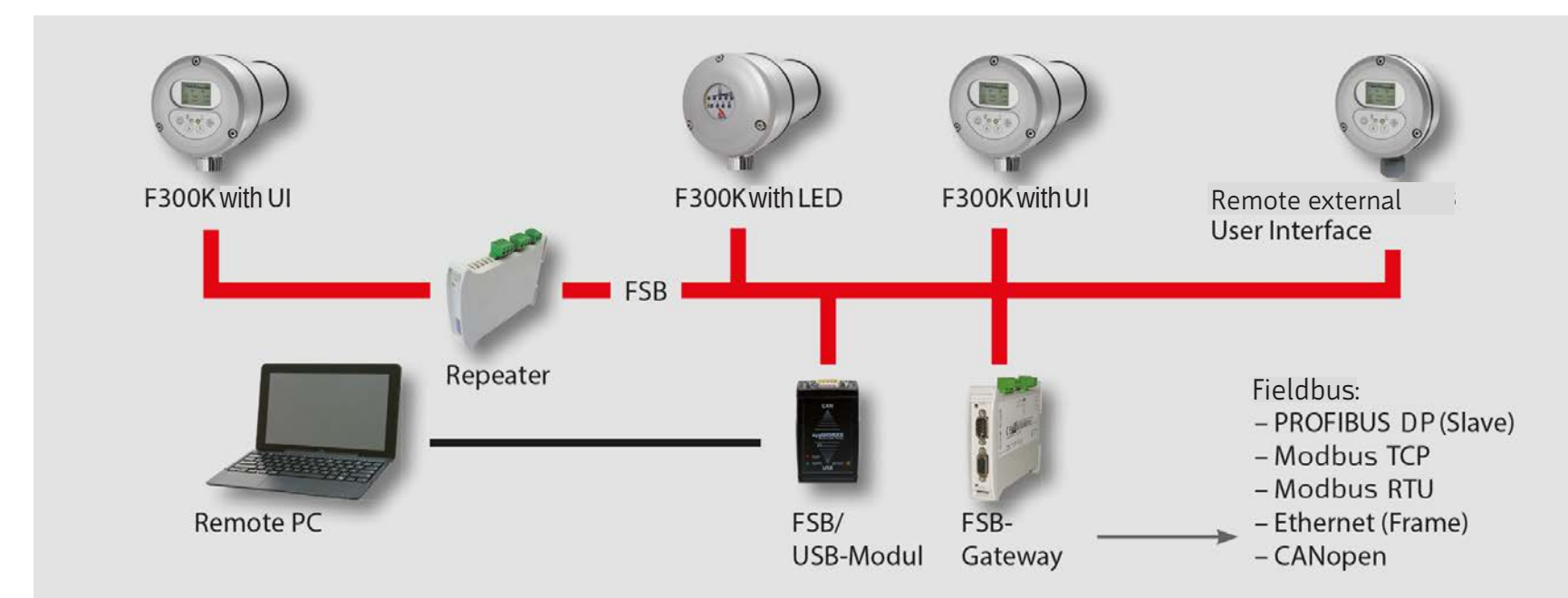
Fig. Example: Networking of several F300K
